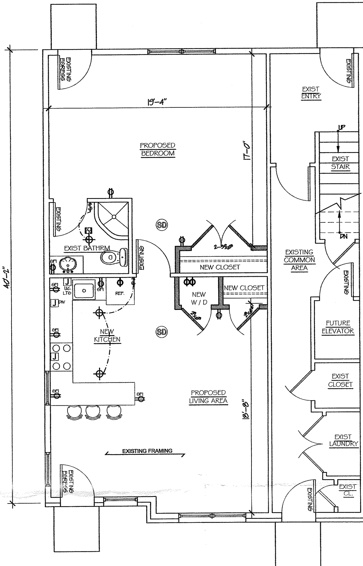
FIRST FLOOR PLAN (649 MAIN STREET) SCALE: 3/16"=1'-0"
