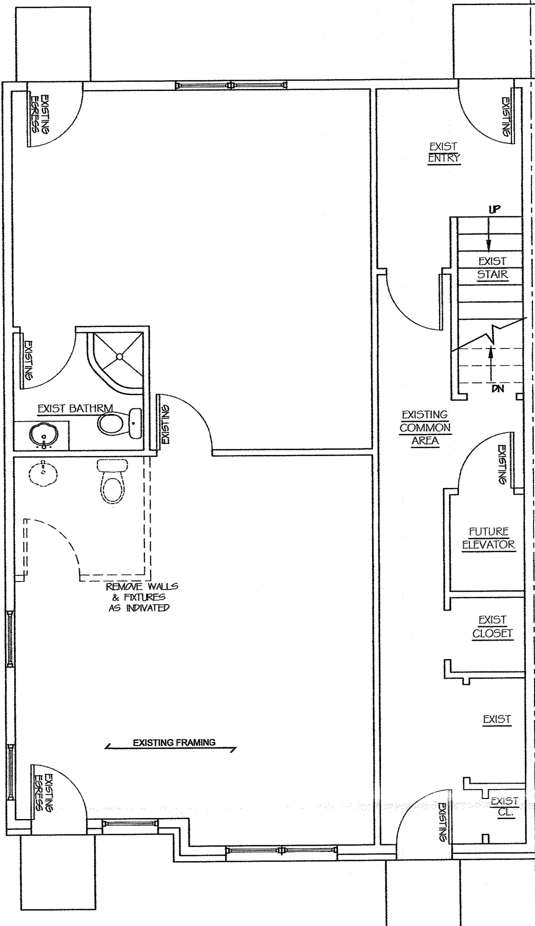
EXISTING/DEMOLITION PLAN (649 MAIN STREET) SCALE: 3/16"=1'-0"
