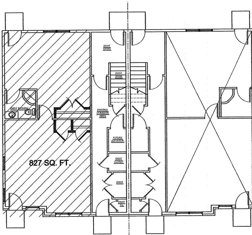
649 MAIN ST KEY PLAN NOT TO SCALE
