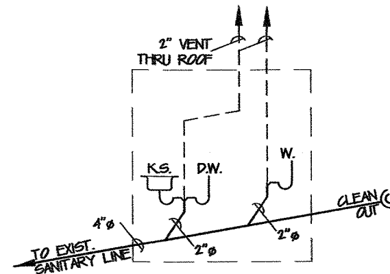
RISER DIAGRAM
