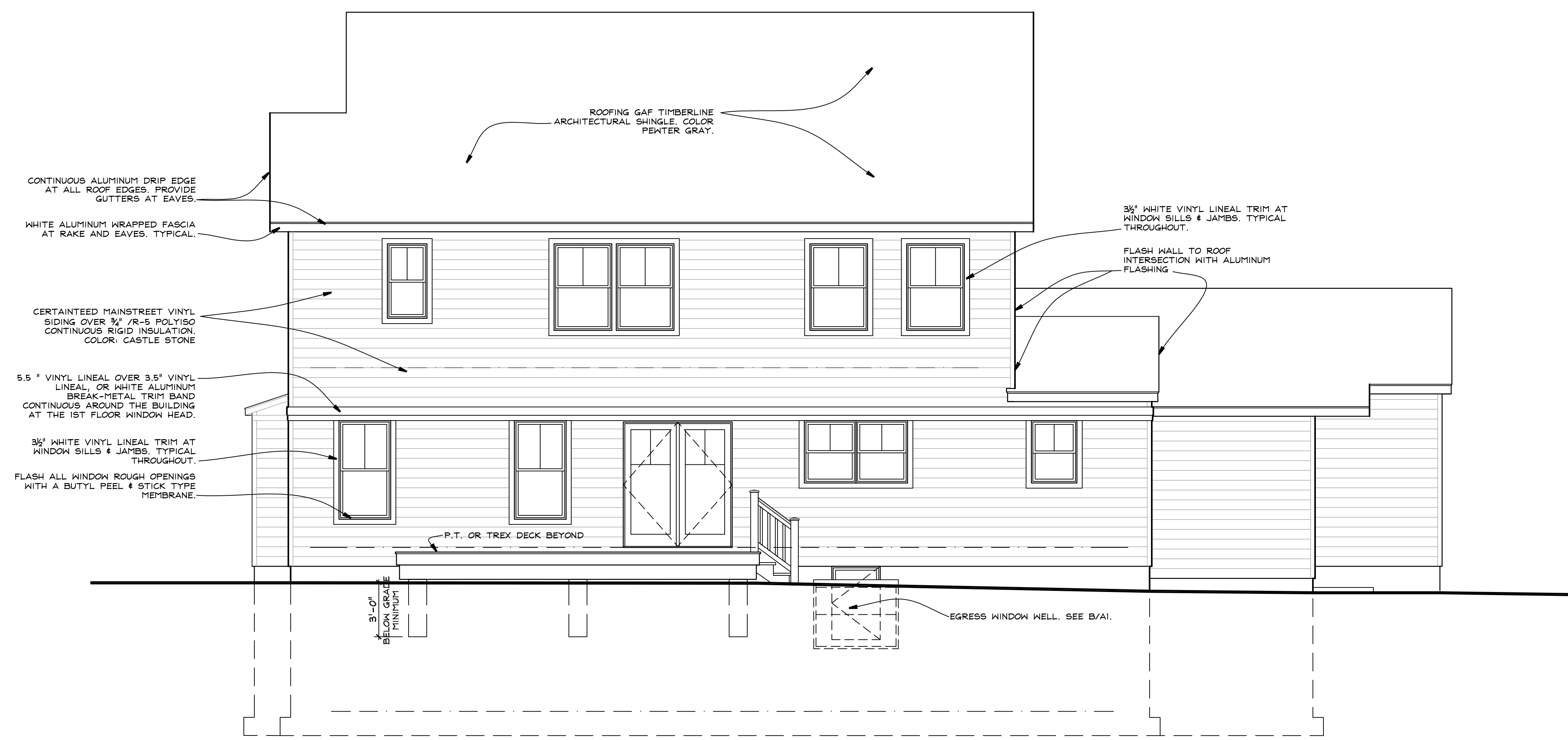
(D) REAR (NORTH) ELEVATION A5 1/4" = 1 FOOT
