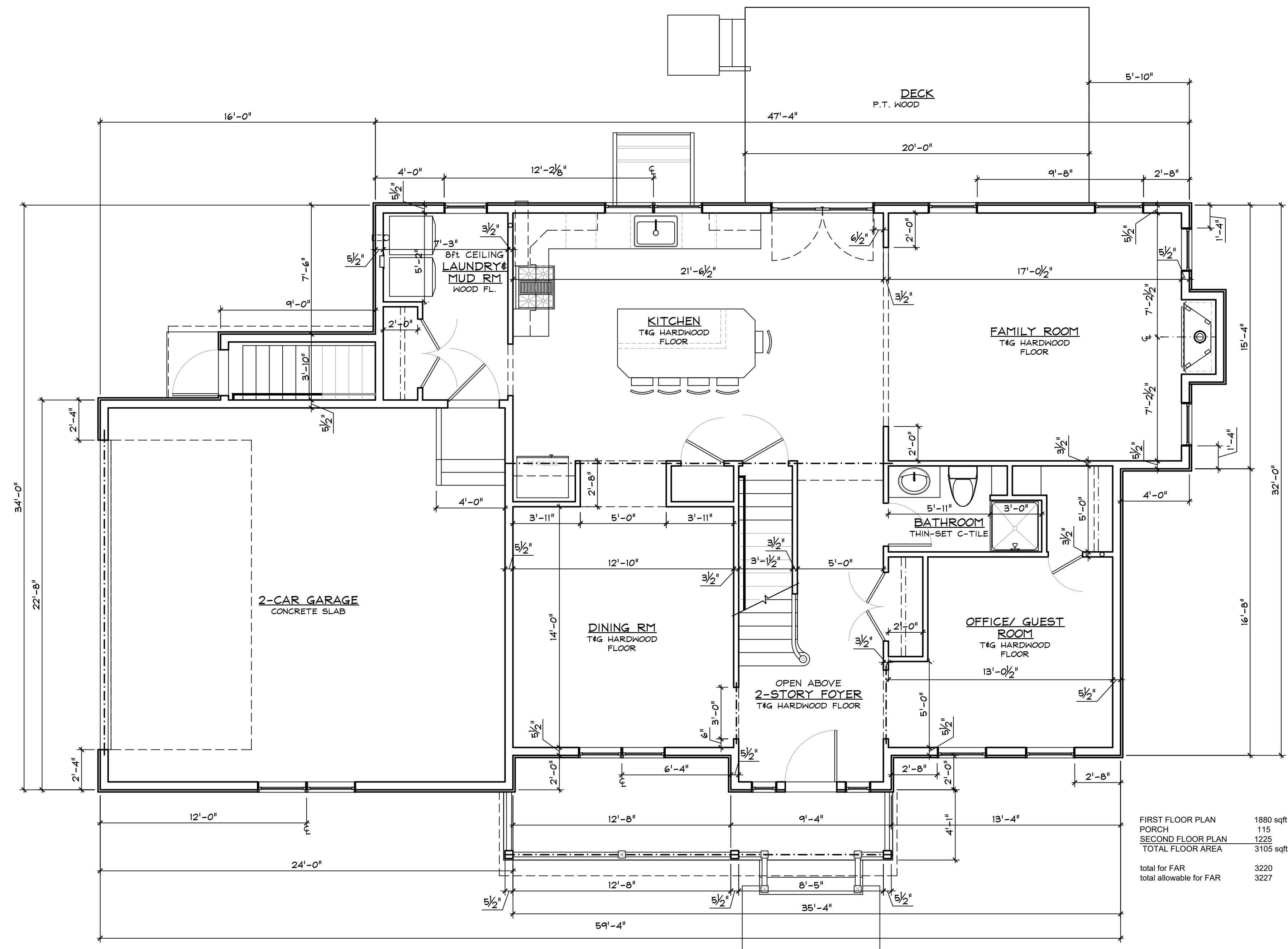
1 FIRST FLOOR PLAN A2 1/4" = 1 FOOT
