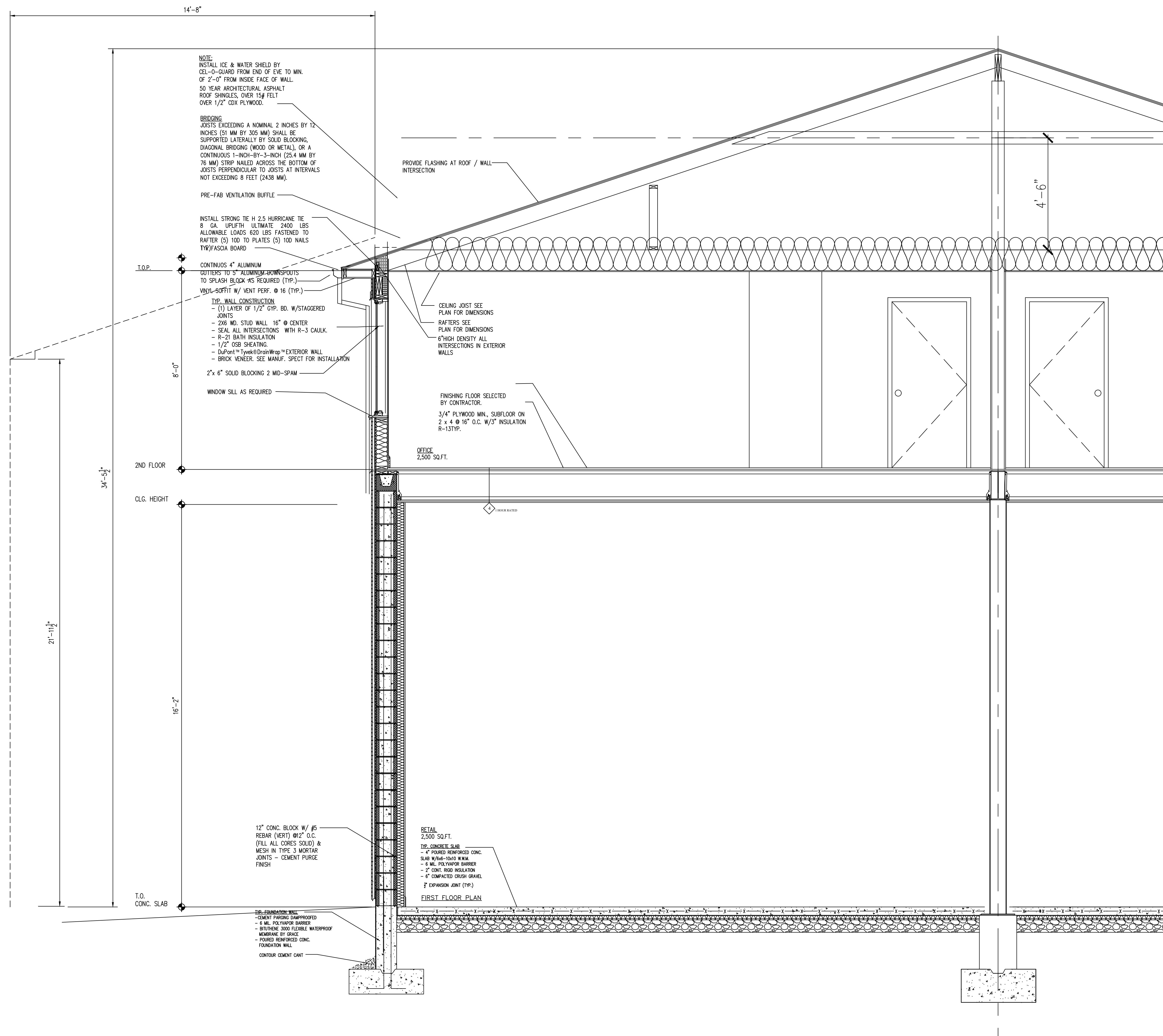
A CROSS SECTION Scale: 3/4"=1'-0"
