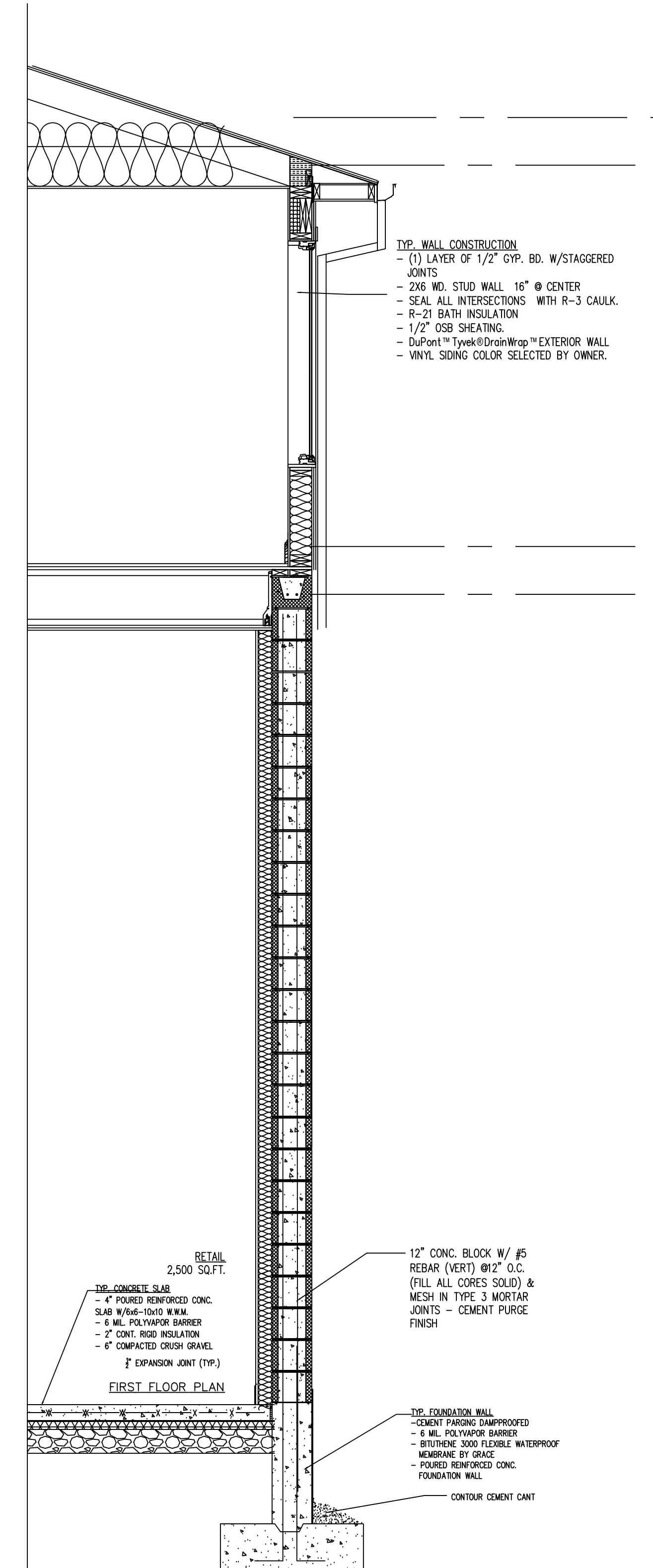
A CROSS SECTION Scale: 1/2"=1'-0"
