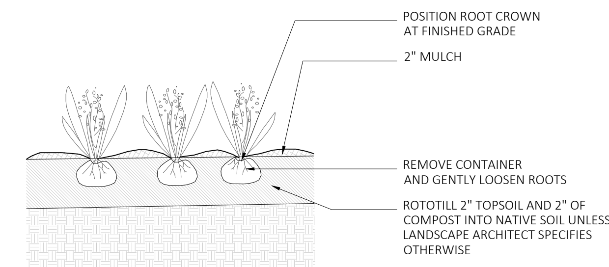
1 GRASS PLANTING DETAIL SCALE: 1/2"=1'
