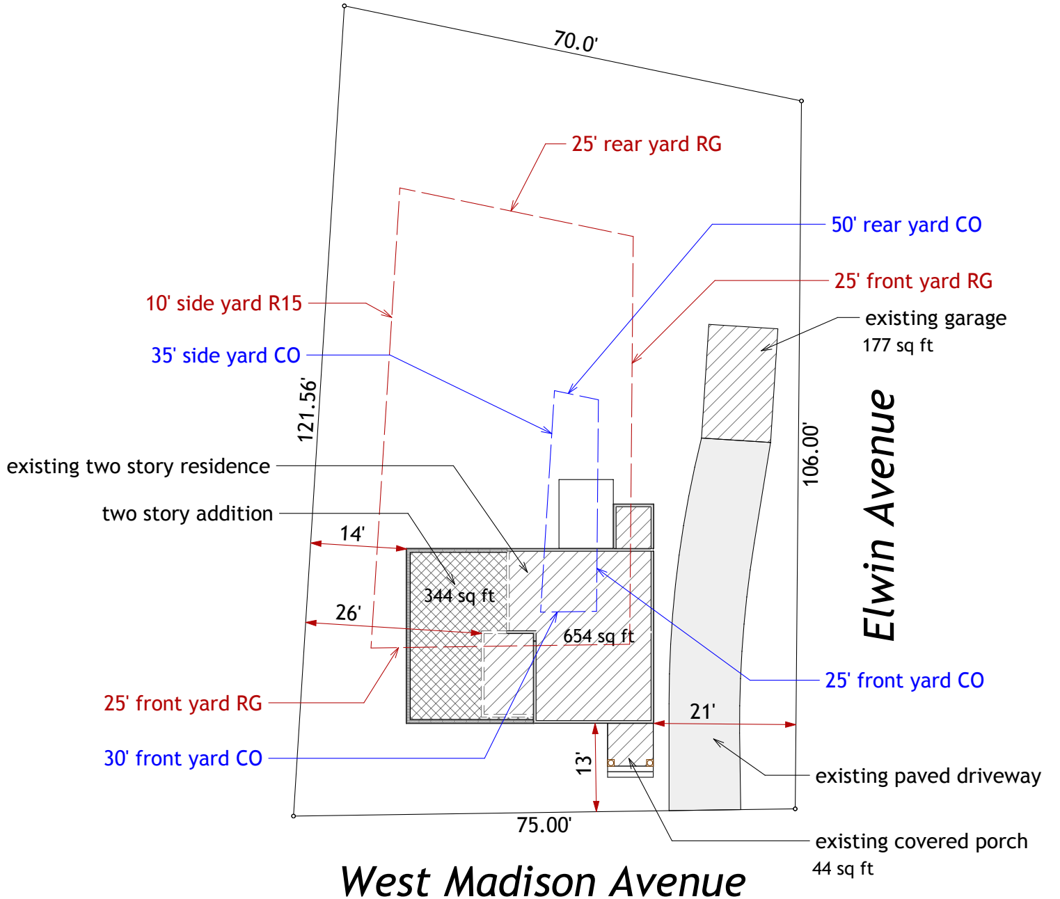
Site Plan
