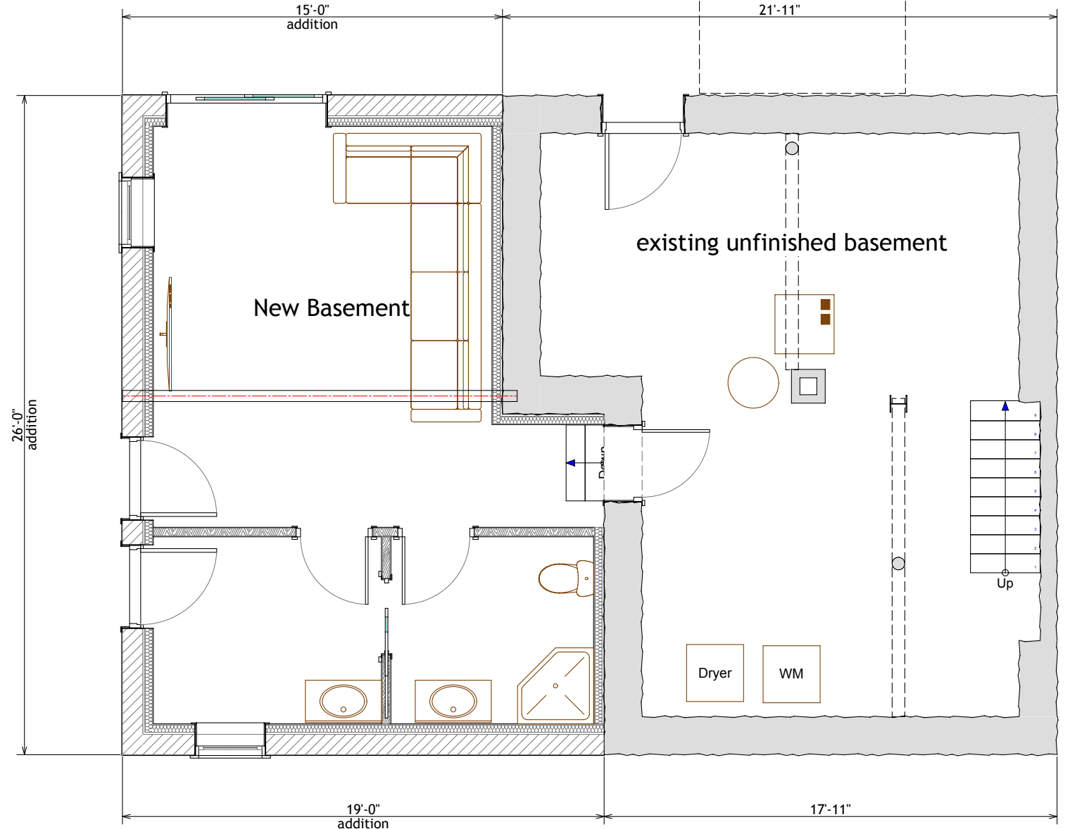
Basement Plan
