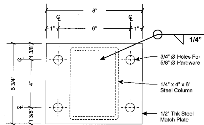
MATCH PLATE DETAIL SCALE: NTS
