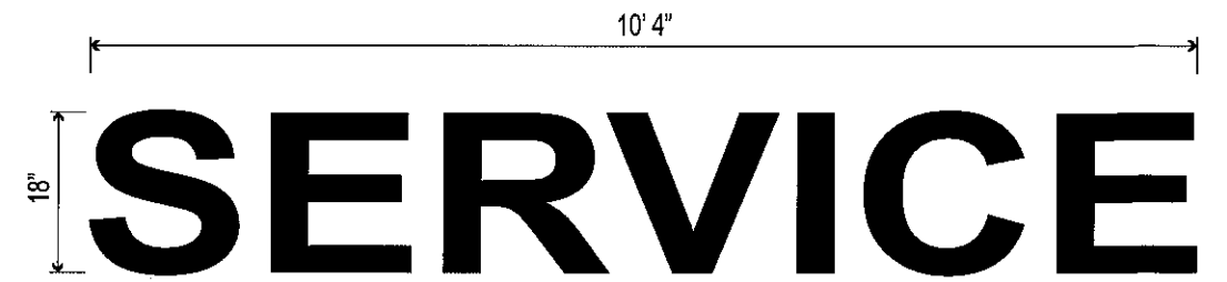
N04 - 18" ILLUM CHANNEL LETTER Scale: 1/2" = 1' 0"
