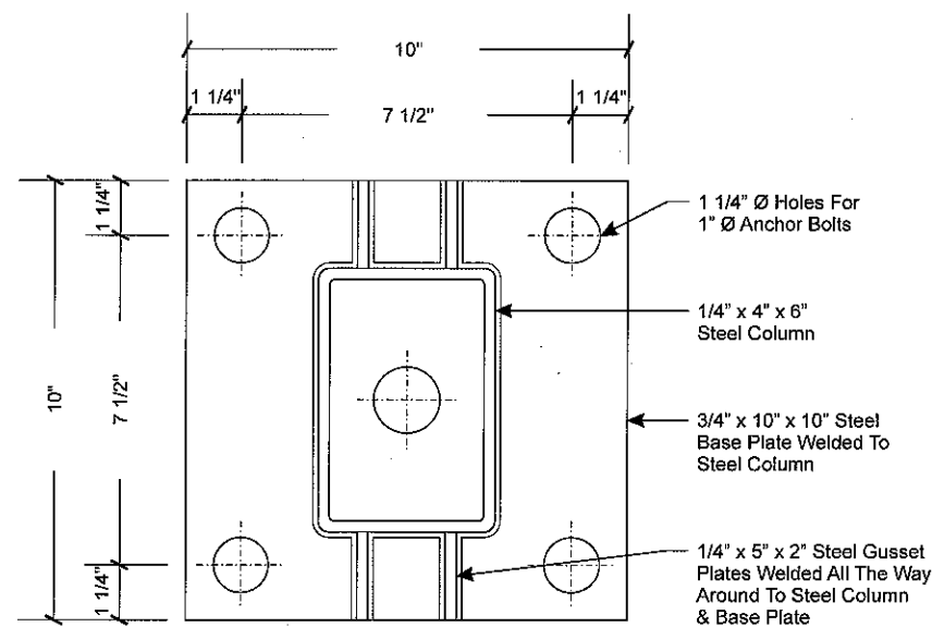
BASE PLATE DETAIL SCALE: NTS
