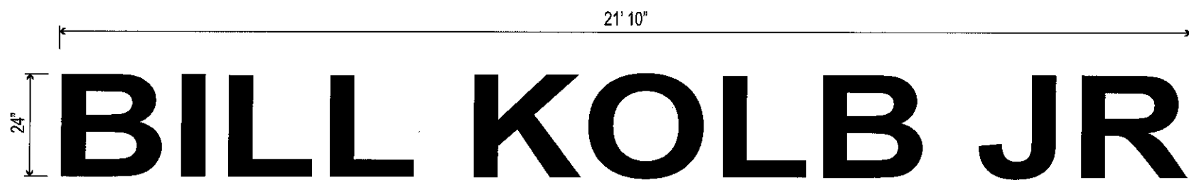
N03 - 24" ILLUM CHANNEL LETTER Scale: 3/8" = 1' 0"
