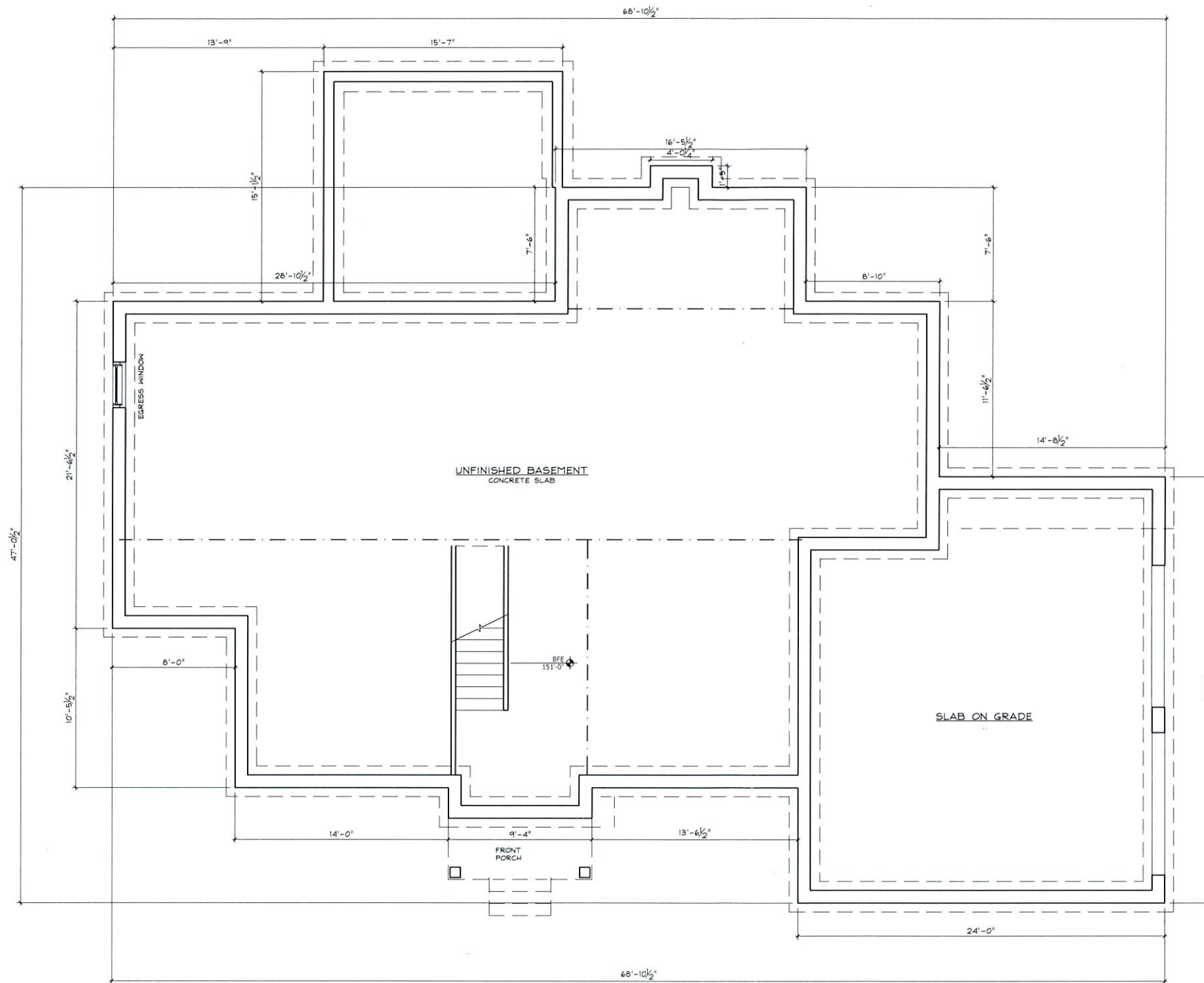
1 FIRST FLOOR PLAN A2 1/4" = 1 FOOT
