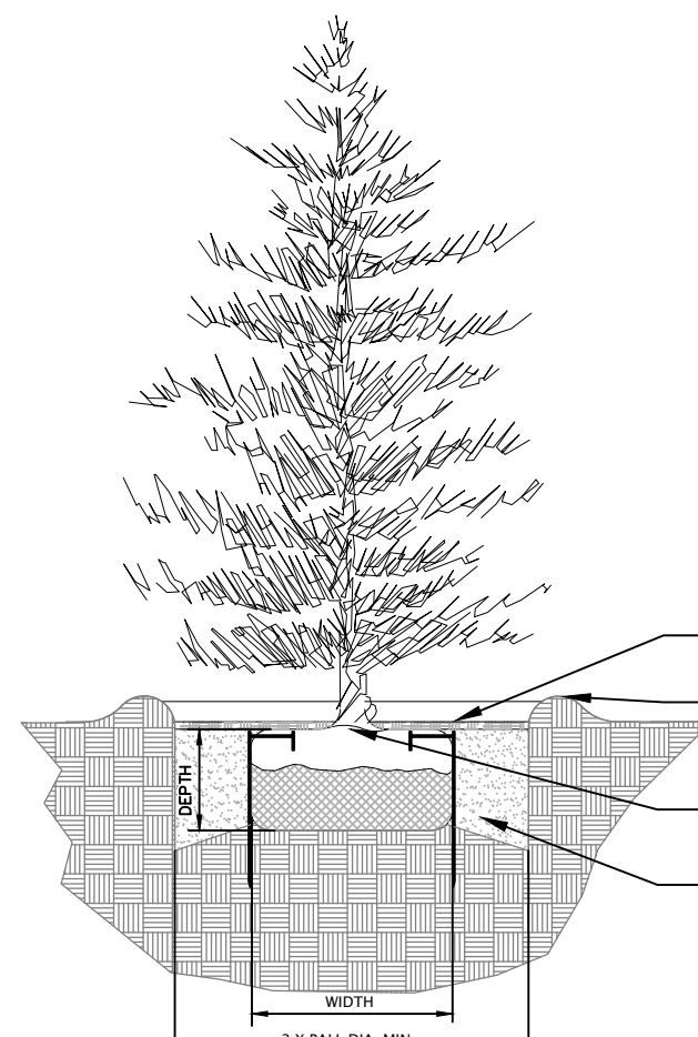
CONIFER PLANTING NOT TO SCALE
