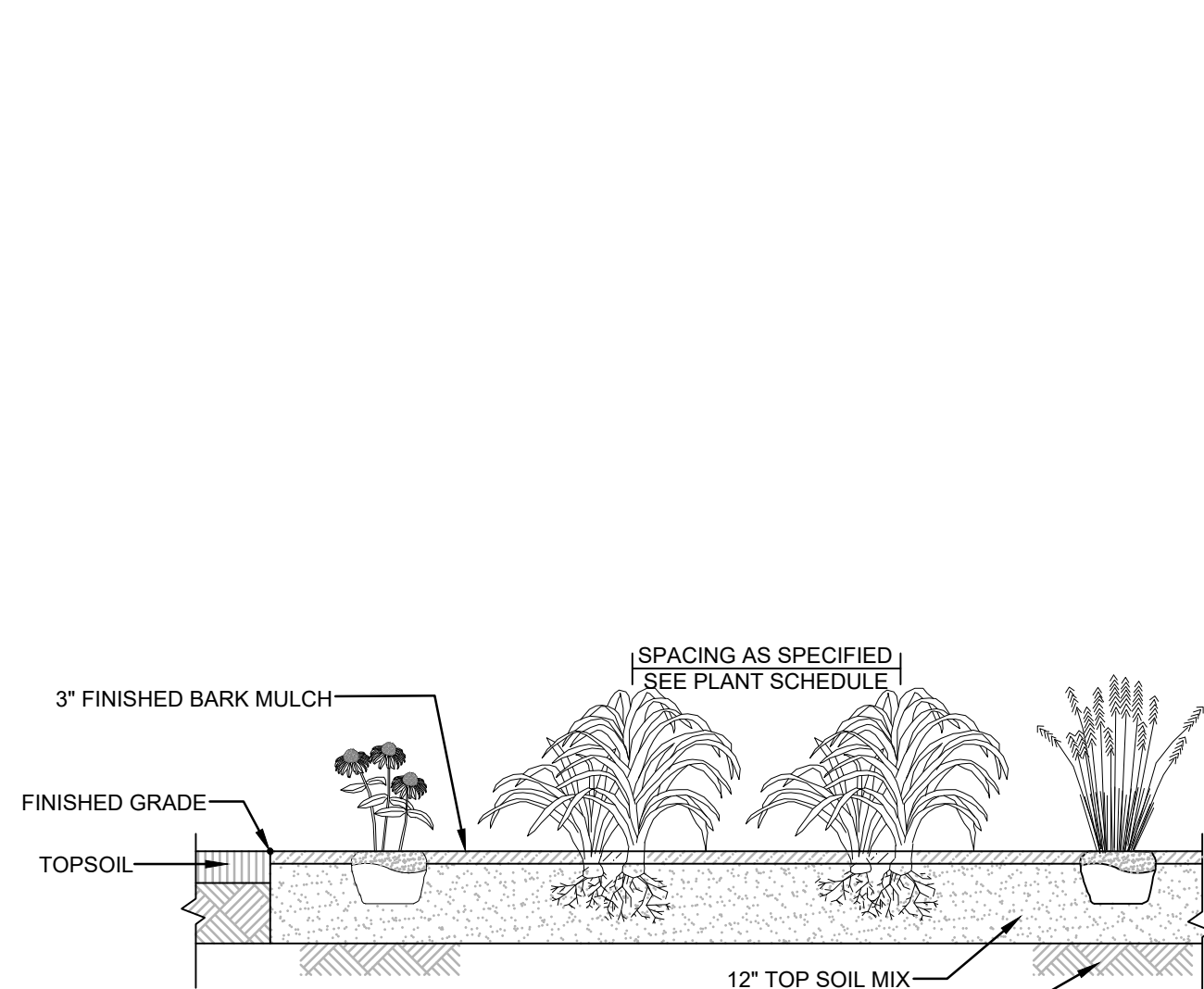
ANNUAL /PERENNIAL/GRASSES/GROUNDCOVER BEDS NOT TO SCALE
