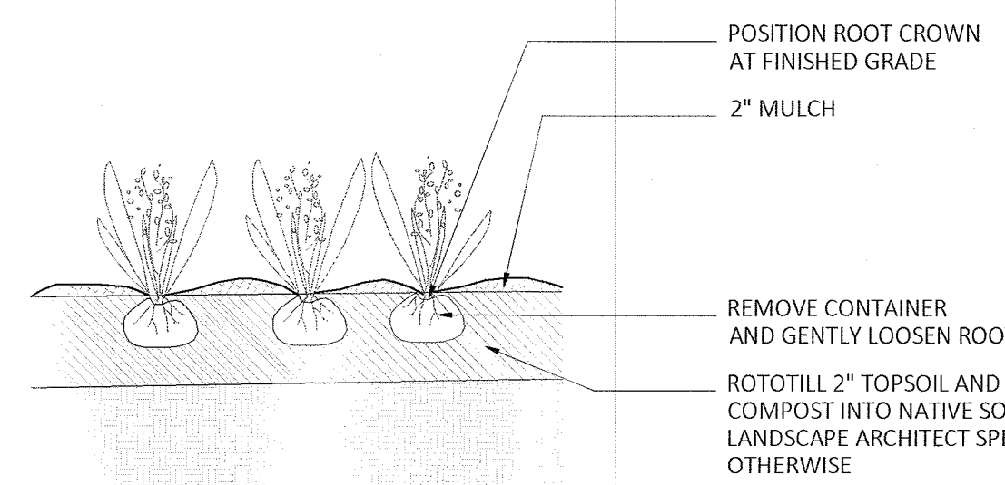
2 GROUND COVER PLANTING SCALE: 1/2"=1'
