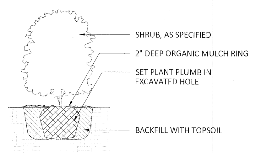
1 SHRUB PLANTING SCALE: 1/2"=1'
