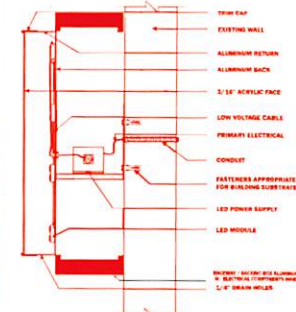
Standard Face Lit - LED Illuminated w/ Raceway
