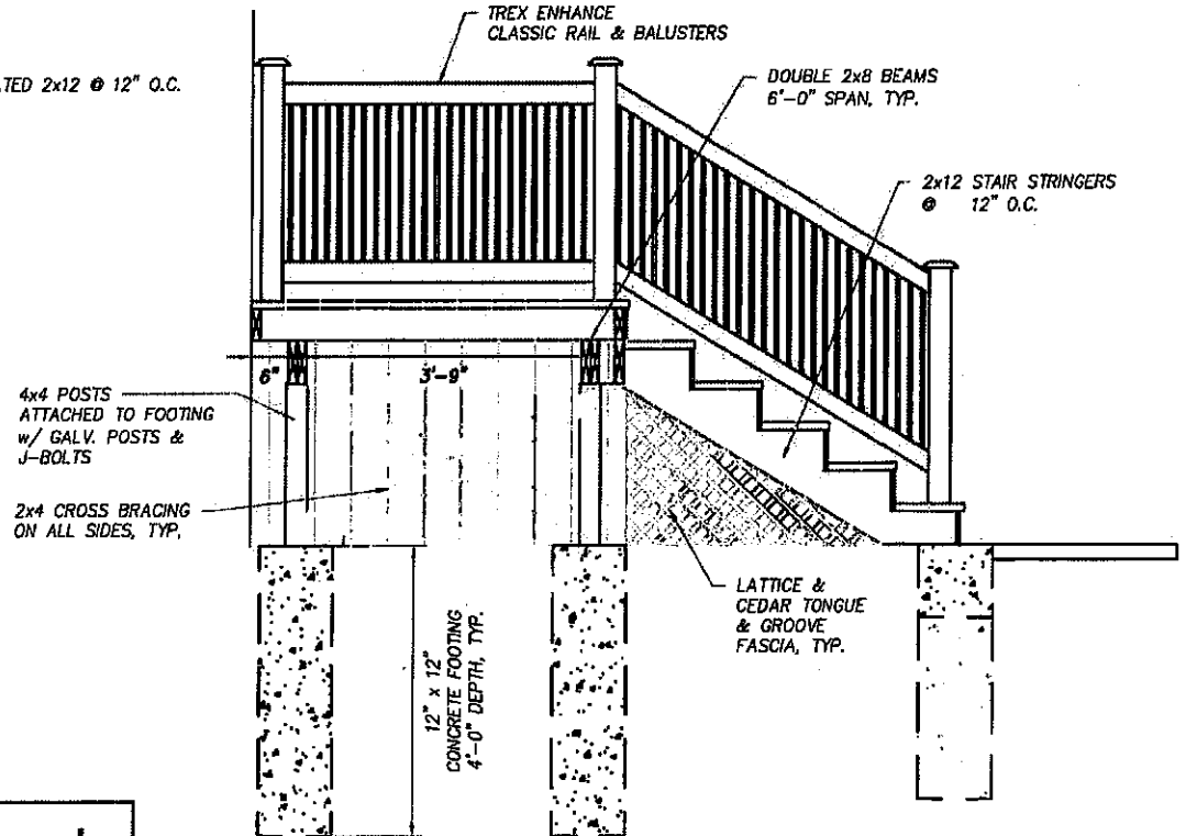
FRONT ENTRY DECK SIDE ELEVATION 3/8" = 1'-0"
