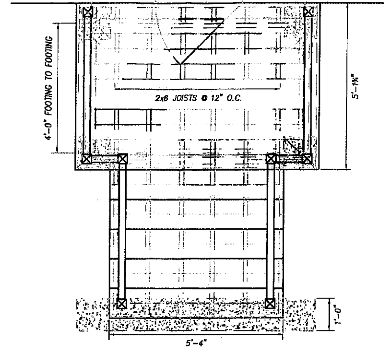
FRONT ENTRY DECK PLAN 3/8" = 1'-0"
