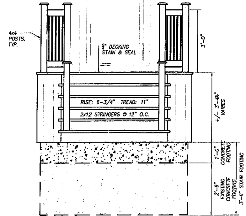
FRONT ENTRY DECK ELEVATION 3/8" = 1'-0"
